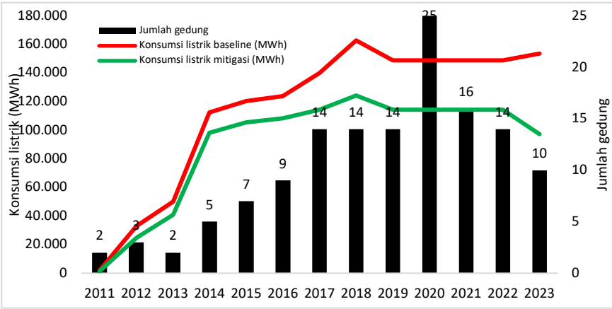
Gambar 4.12 Penerapan green building di gedung komersial
